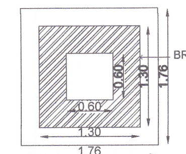
FOR PIPES DIAMETER UPTO 450mm UPTO DEPTH OF 1.5 M (C2)
