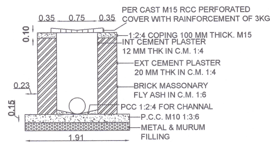
FOR LINE WITH PIPE DIAMETER UPTO 750 MM
