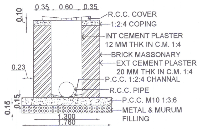
FOR LINE WITH PIPE DIAMETER UPTO 600 MM
