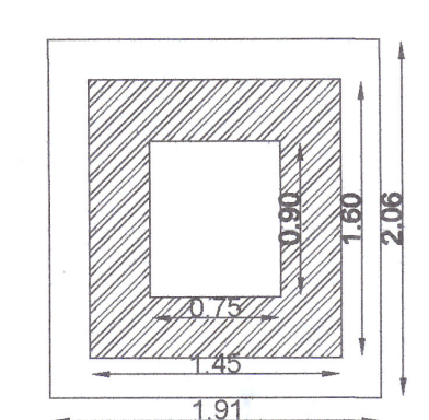
FOR PIPES DIAMETER ABOVE 450 MM TO 600 MM UPTO DEPTH OF 1.5 M (C1)
