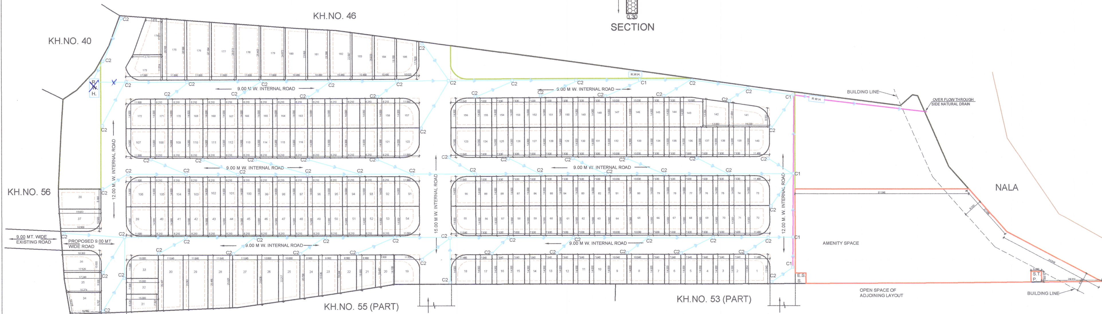
STORM WATER DRAIN LINE PLAN SCALE : 1:1000
